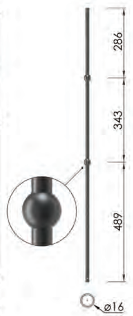
Round Double Sphere 1118 x ø16mm RDS-MX
