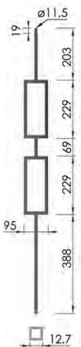
Double Rectangle 1118 x 95 x 12.7mm SDRS-MX
