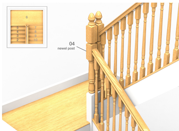
9. Half turn with landing
