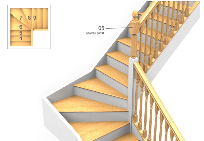
8. Quarter turn with 3 winders
