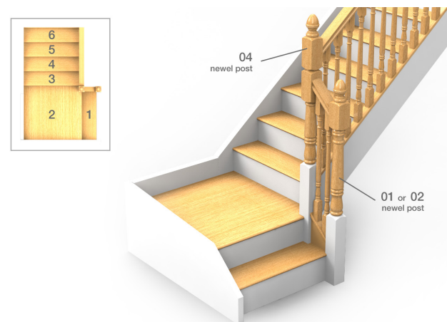
5. 90° turn with flush tread
