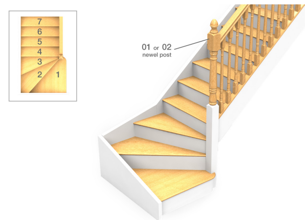
4. 90° winder with Bullnose tread
